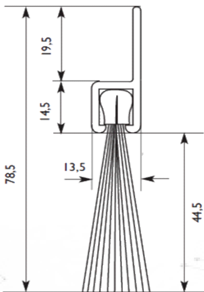
ELASTO-SEAL GS (Nylon noir, \varnothing : 0,508 mm)
