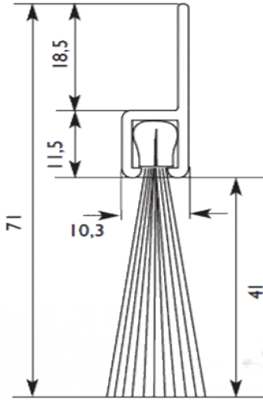
ELASTO-SEAL E (Nylon noir, \varnothing : 0,305 mm)
