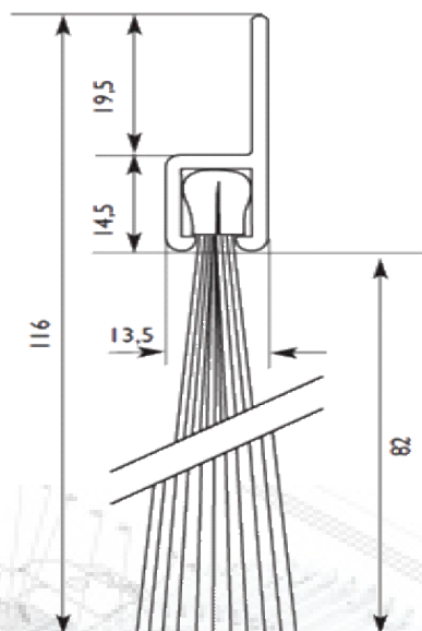
ELASTO-SEAL GSX (Nylon noir, \varnothing : 0,508 mm)
