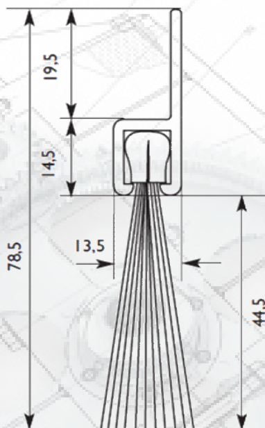
ELASTO-SEAL GW (Nylon noir, \varnothing : 0,610 mm)
