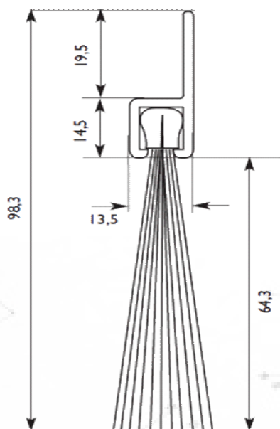
ELASTO-SEAL GM (Nylon noir, \varnothing : 0,330 mm)
