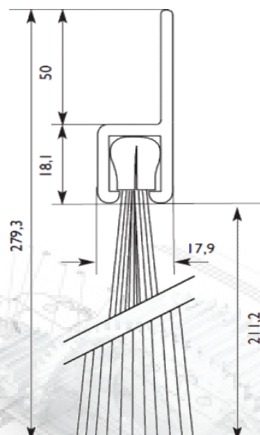
ELASTO-SEAL H (Nylon noir, \varnothing : 0,889 mm)
