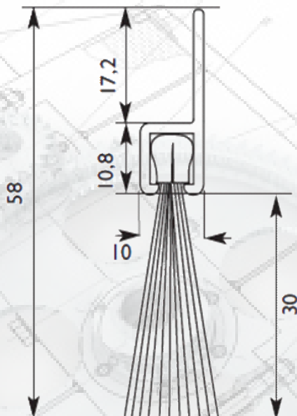
ELASTO-SEAL DX (Nylon noir, \varnothing : 0,203 mm)
